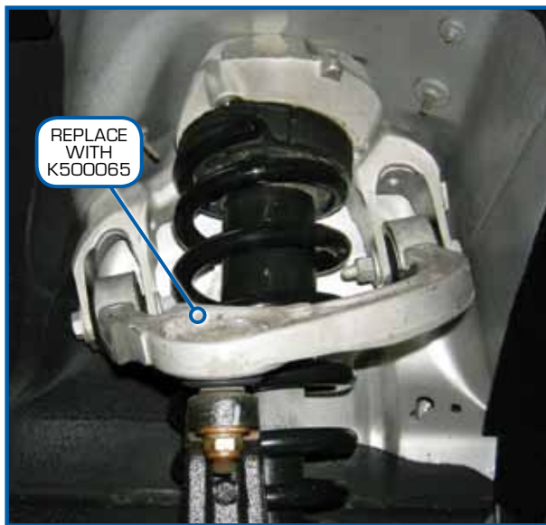
Upper Control Arm/Spring Mount Assembly
